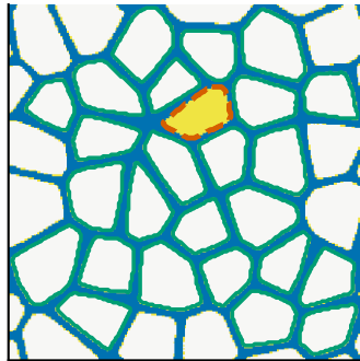
(b) \varepsilon = 0.10
