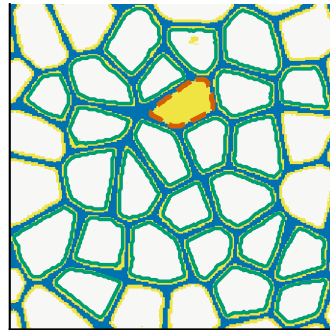
(c) \varepsilon = 0.315
