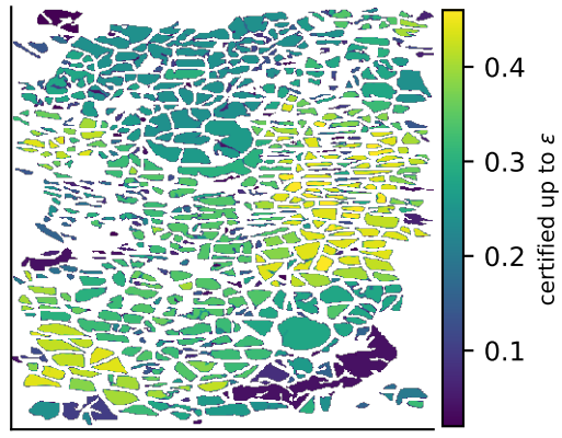
per-tessera certified budget \varepsilon^* (topological: wall OR interior)
