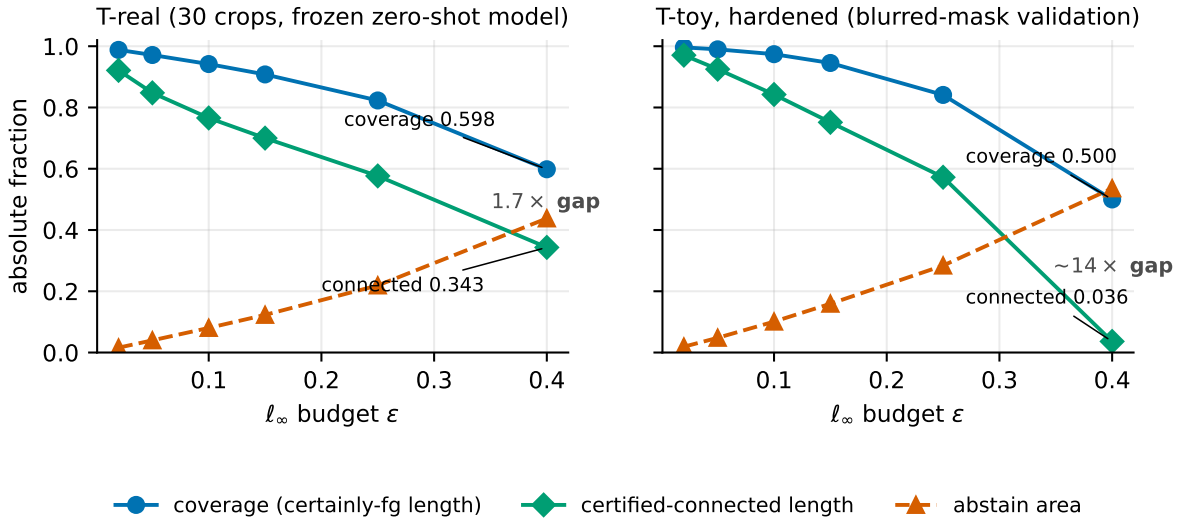
Figure 7: Certified fractions vs. \varepsilon , both tracks (coverage, certified-connected length, abstain). Left (T-real, 30 crops): the coverage-vs-connectivity gap is a modest 1.7\times at \varepsilon = 0.40 (0.598 vs 0.343) — the confident model keeps most segments entirely inside CERT_FG. Right (T-toy): the same gap collapses to \sim 14\times (0.500 vs 0.036), an artifact of the blurred toy maps whose skeletons fragment en masse . Same three series, same y -scale; the panels’ contrast is the point (§5.2).
