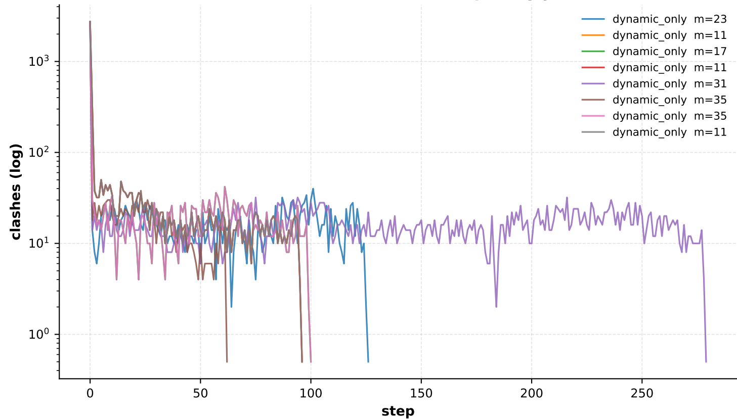
hec-s-92: clashes over steps (log y)
