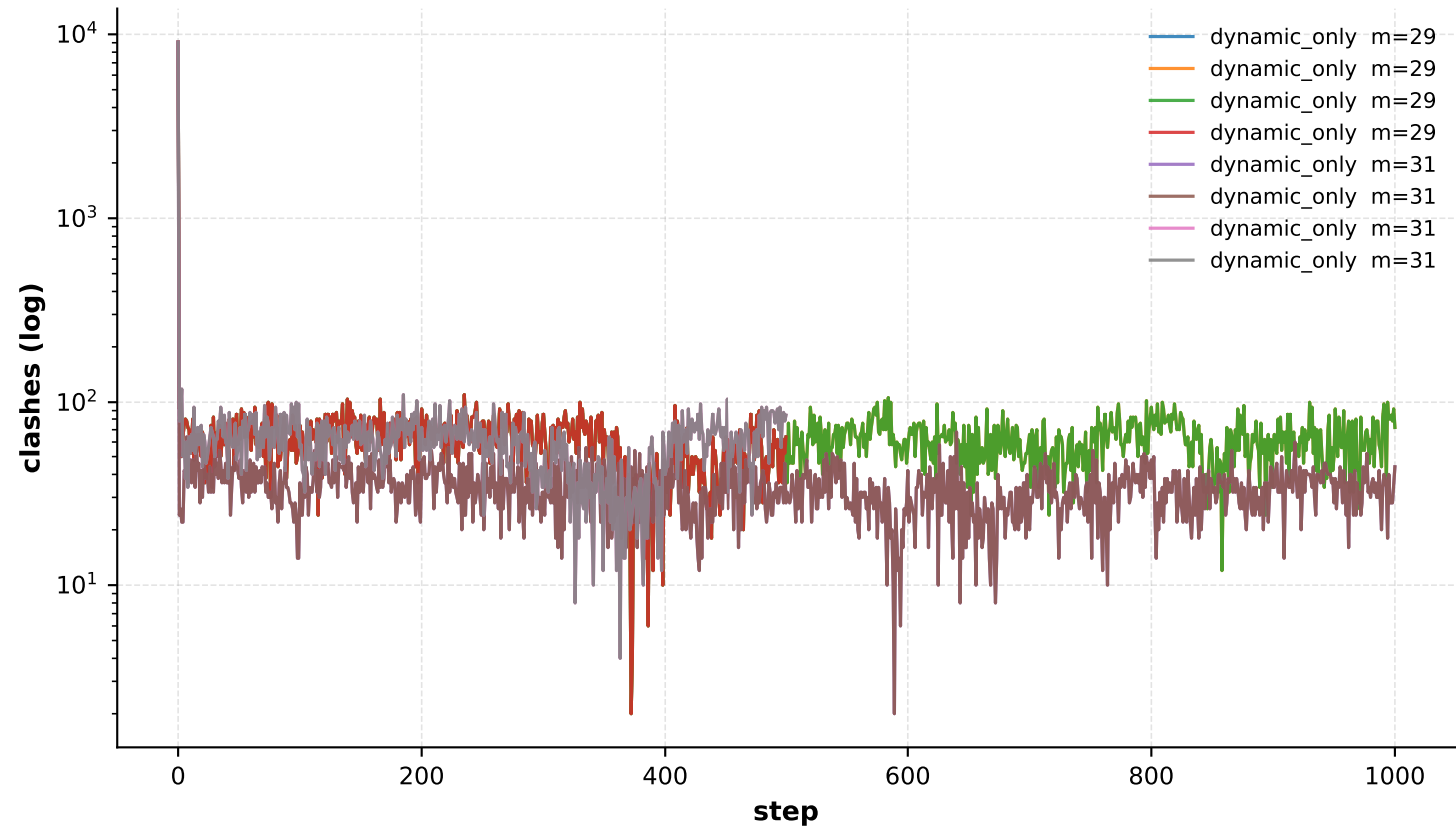
lse-f-91: clashes over steps (log y)
