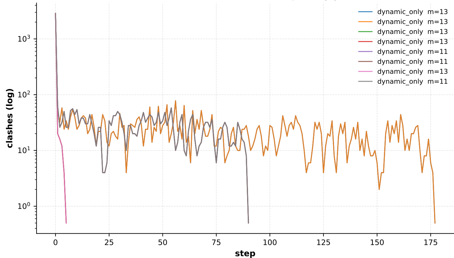
ute-s-92: clashes over steps (log y)
