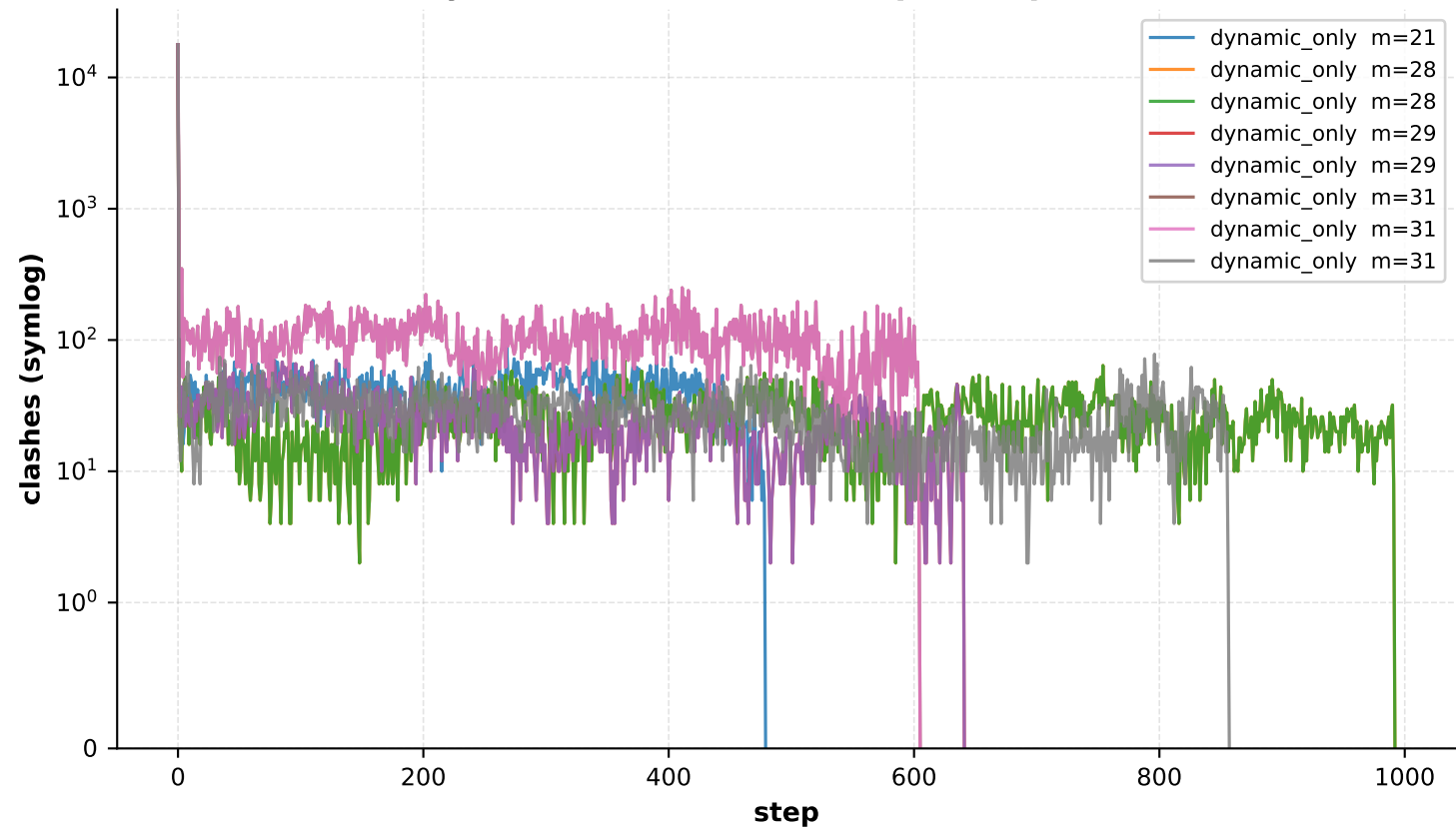
rye-s-93: clashes over steps — top runs
