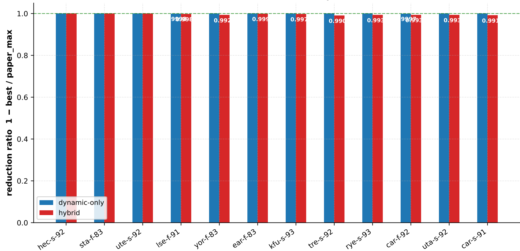
Improvement Ratio Compared to Paper Max Clashes (1.0 = zero clashes achieved — fully conflict-free)
