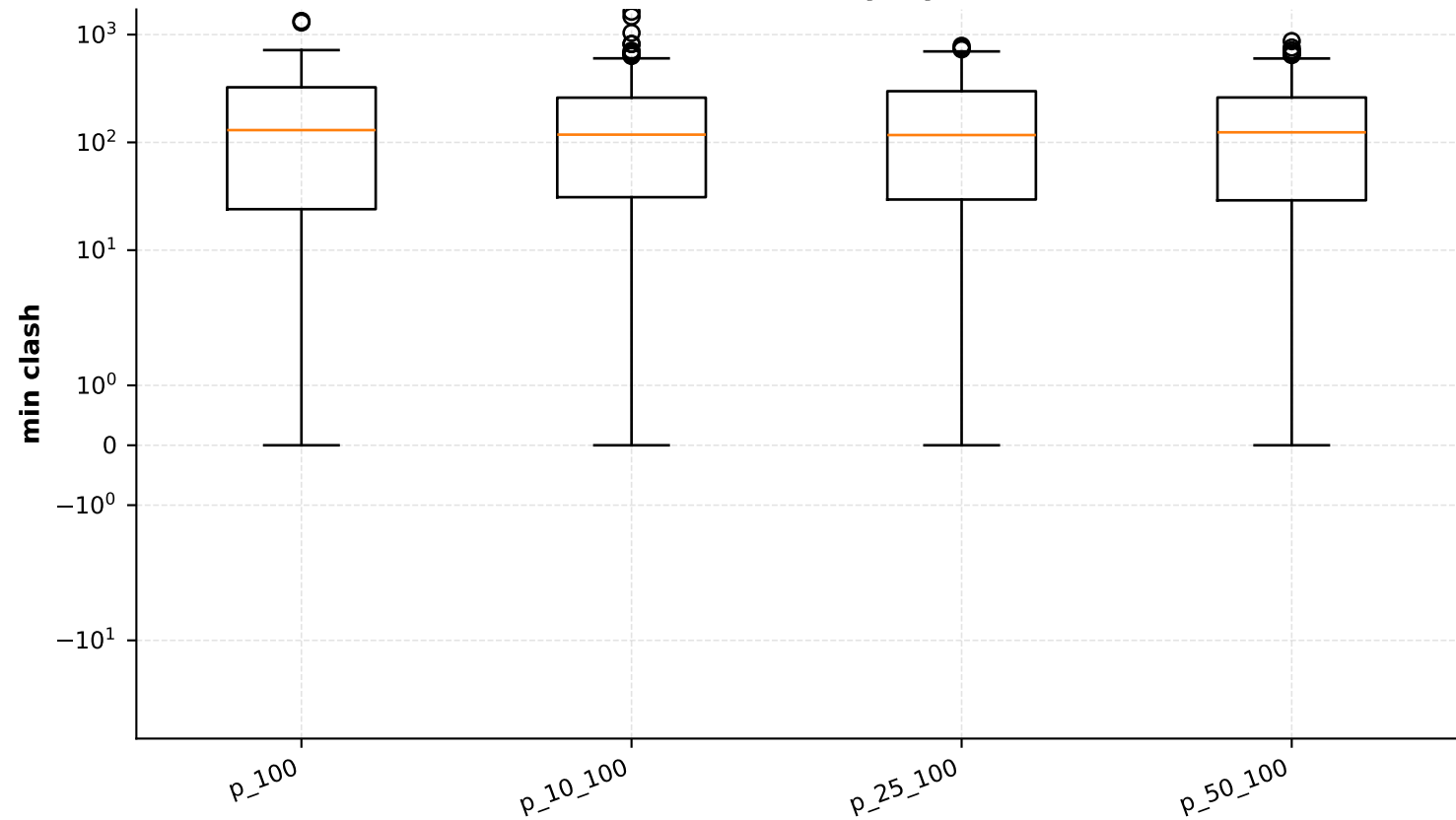
Min Clash Distribution by Hybrid Pattern
