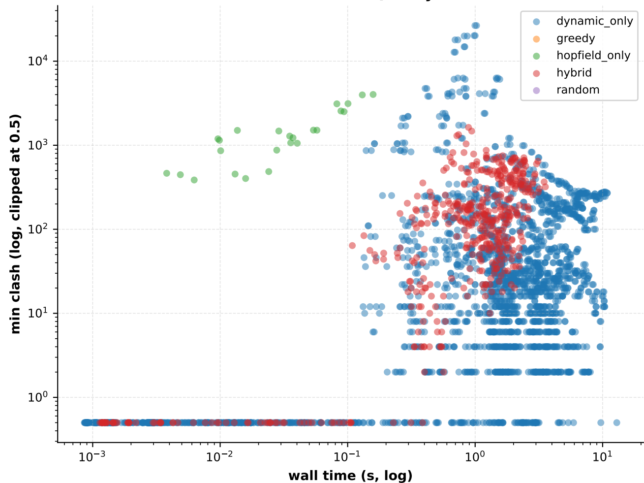
Runtime vs Quality
