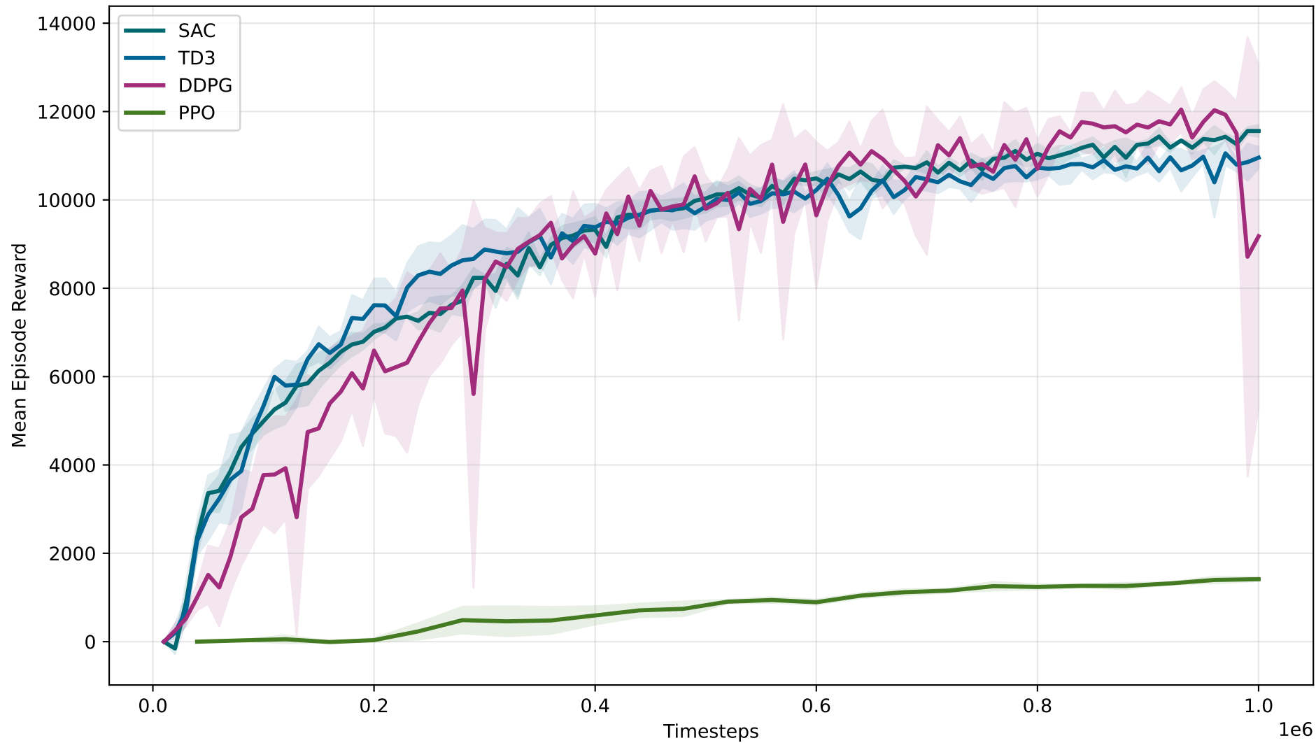
HalfCheetah-v5: SAC vs. TD3 vs. DDPG vs. PPO
