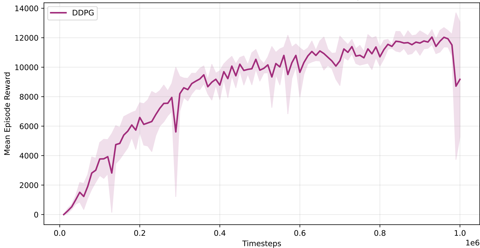
HalfCheetah-v5: DDPG Reward vs. Timestep
