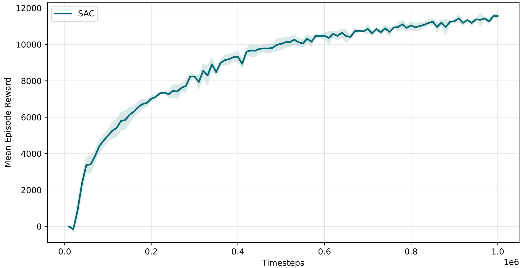
HalfCheetah-v5: SAC Reward vs. Timestep
