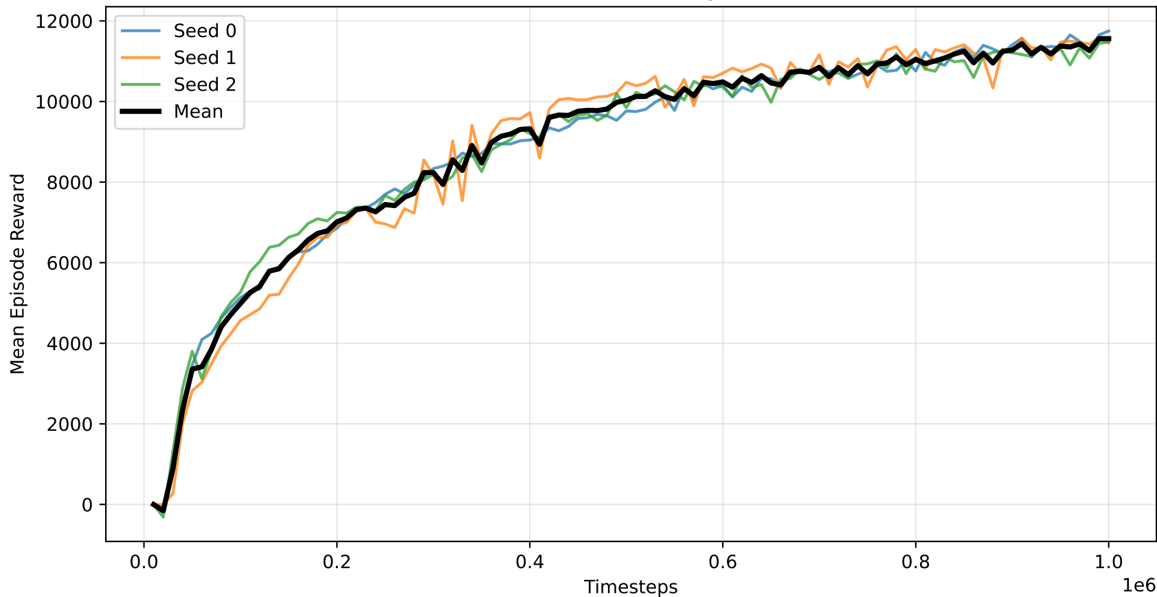
SAC: Per-Seed Learning Curves
