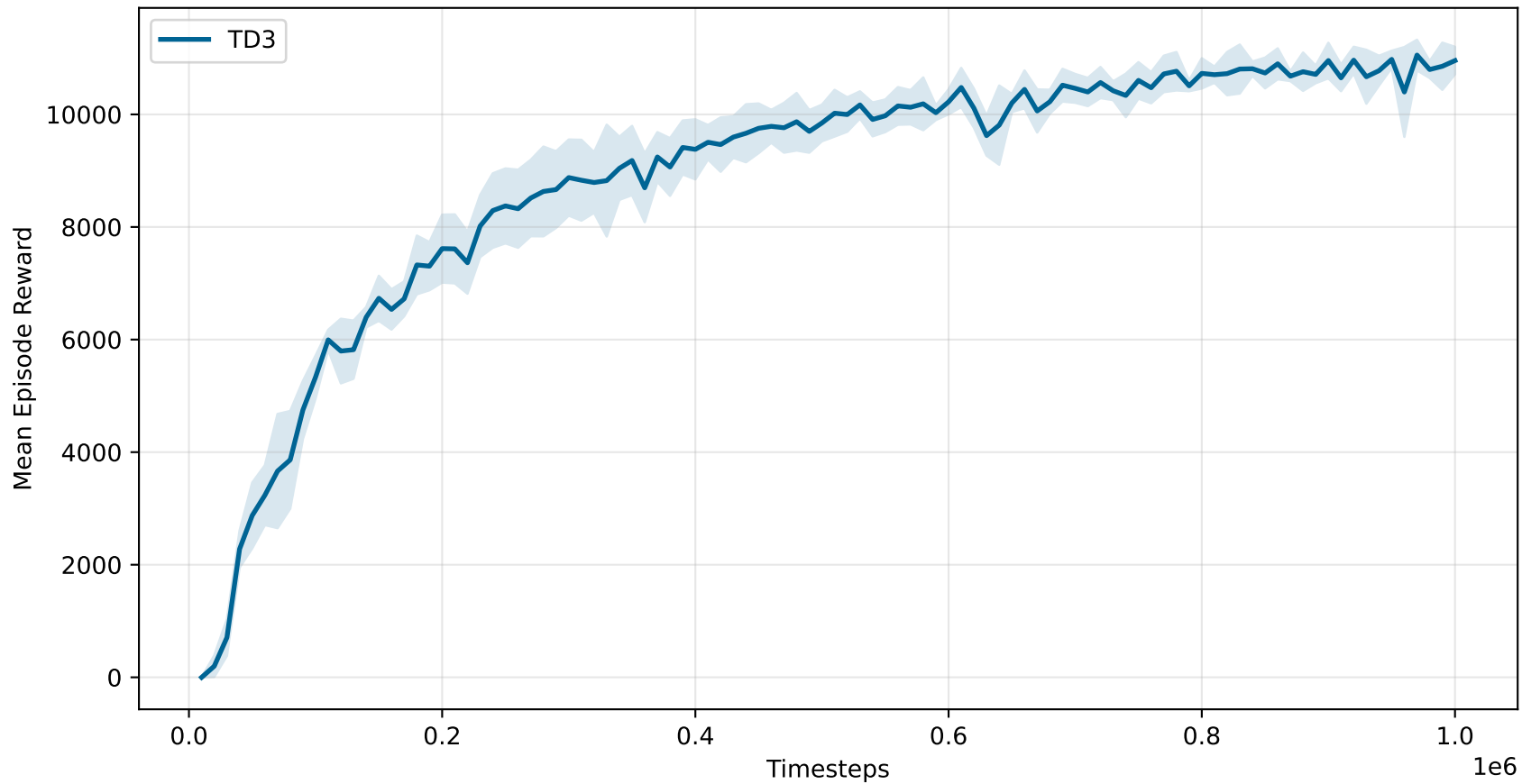
HalfCheetah-v5: TD3 Reward vs. Timestep
