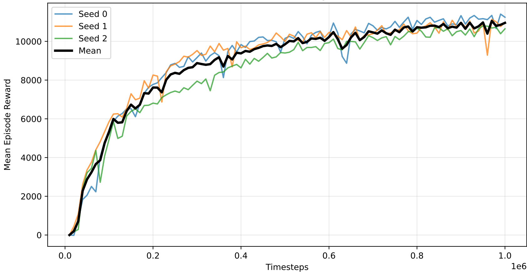
TD3: Per-Seed Learning Curves
