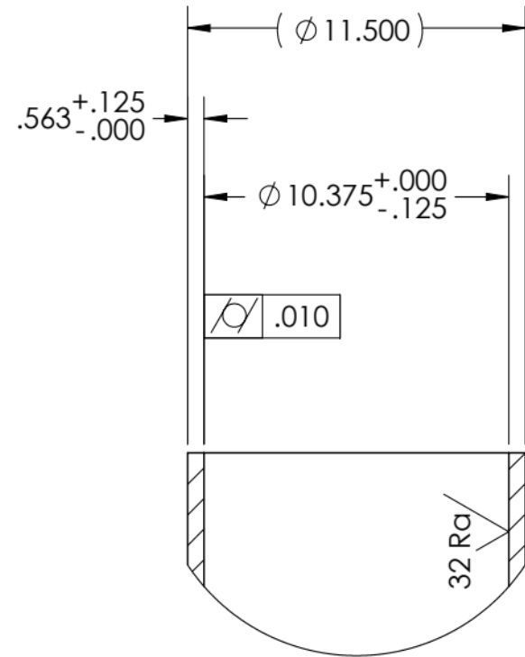
DETAIL B SCALE 1 : 5.9
