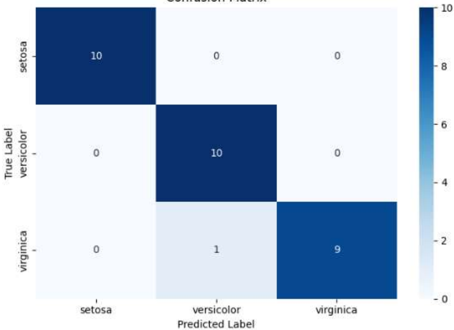
Confusion Matrix
