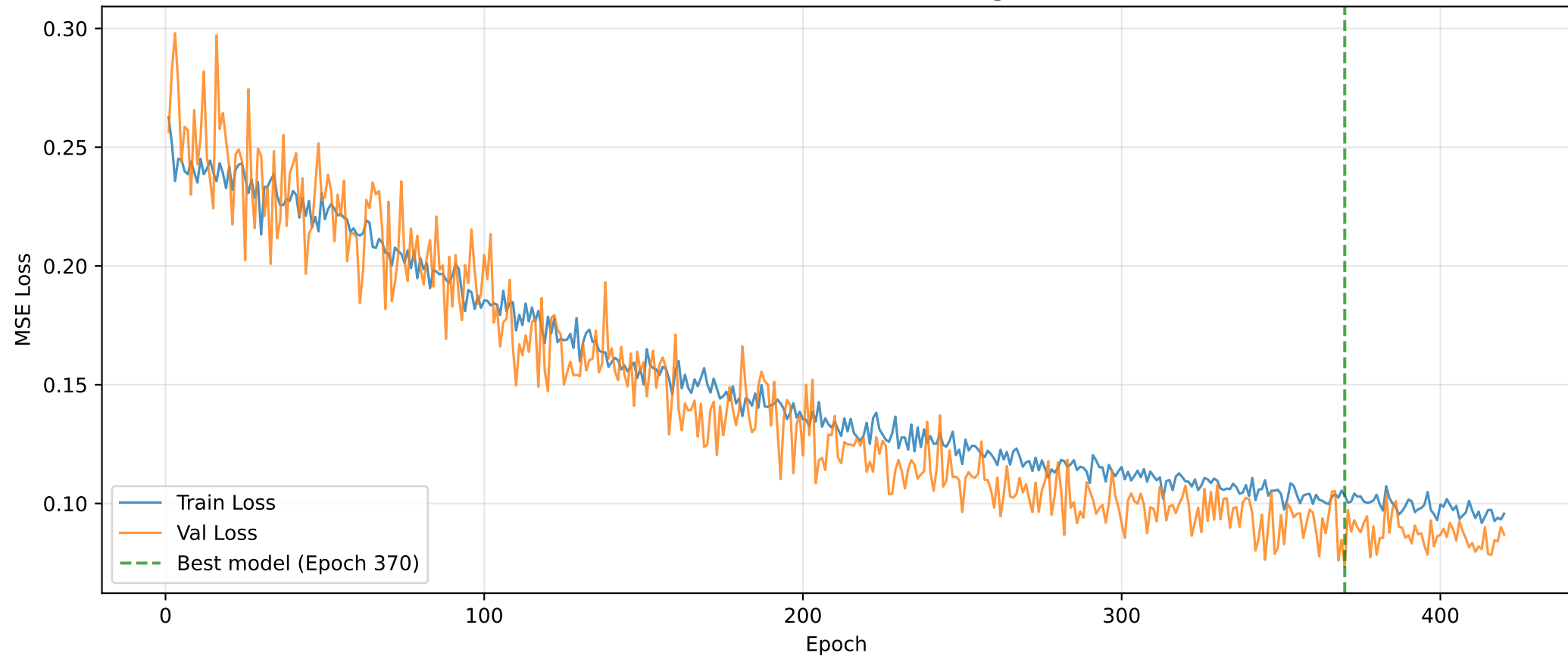
Conditional DDPM — Training Curves
