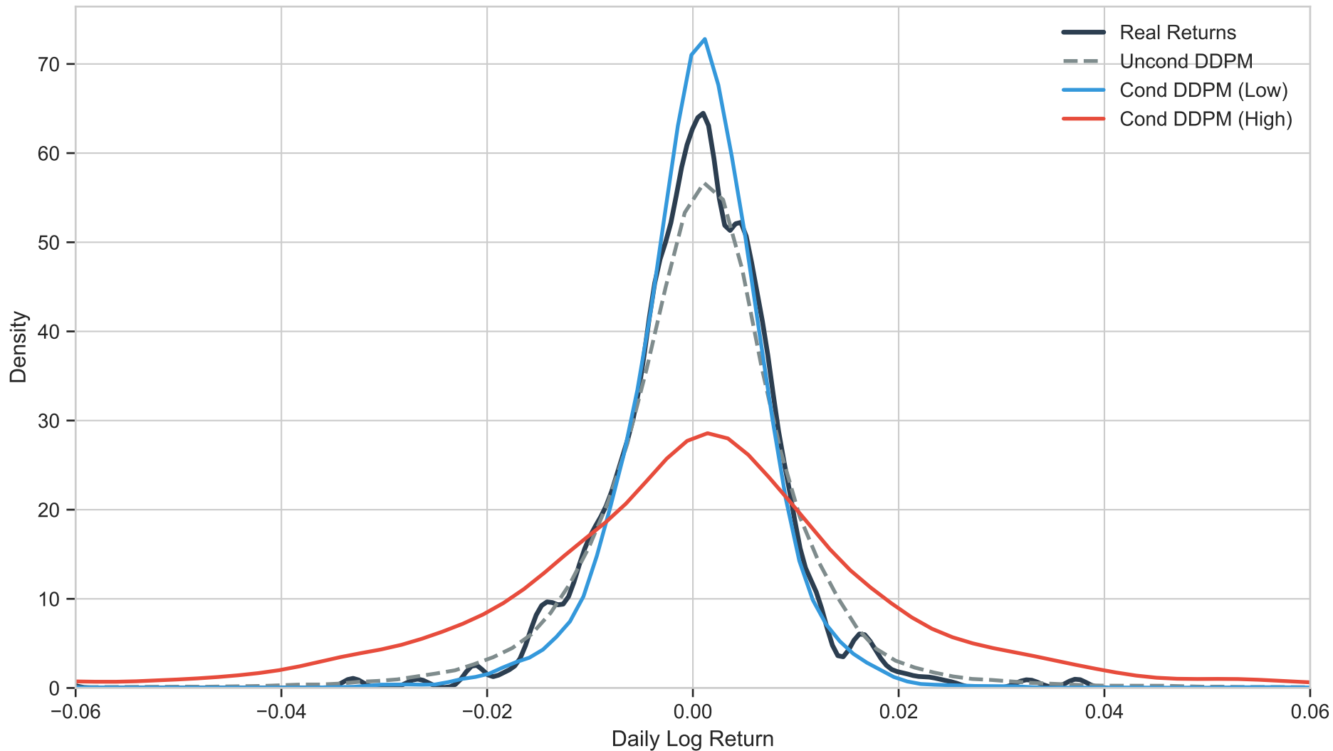
Kernel Density of Daily Returns
