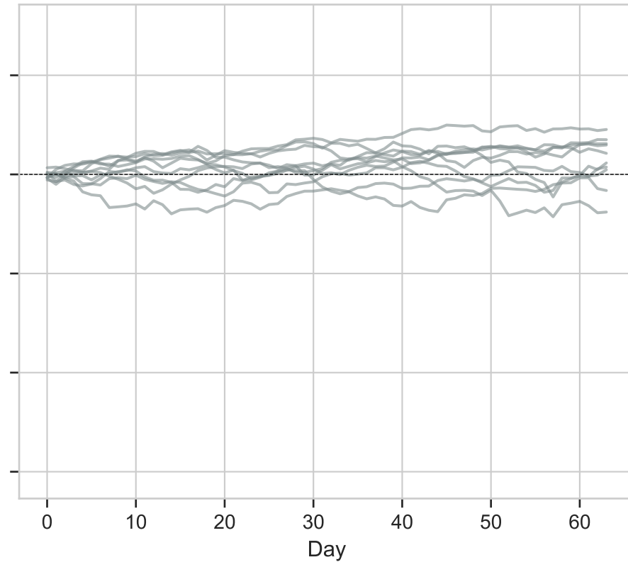
Unconditional DDPM
