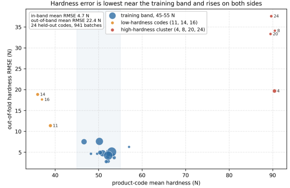
(b) Out-of-fold hardness error for each held-out product code against that code's mean hardness. Error is lowest near the centre of the training distribution and rises on both sides.
