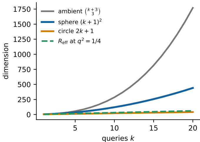
Algebraic and effective support
