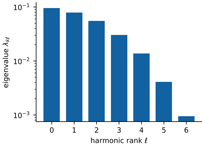
Bell-frame spectrum: k = 6, q^2 = 1/4
