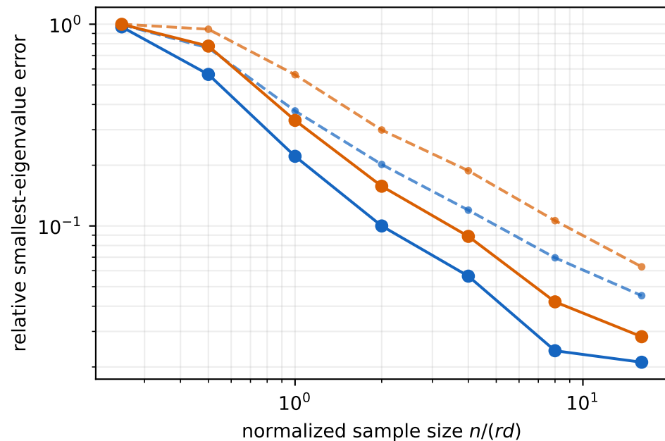
Finite-sample resolution ( d = 12, r = 6, 320 repetitions)
