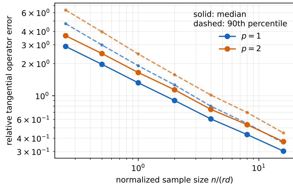
Finite-sample resolution ( d = 12, r = 6, 320 repetitions)
