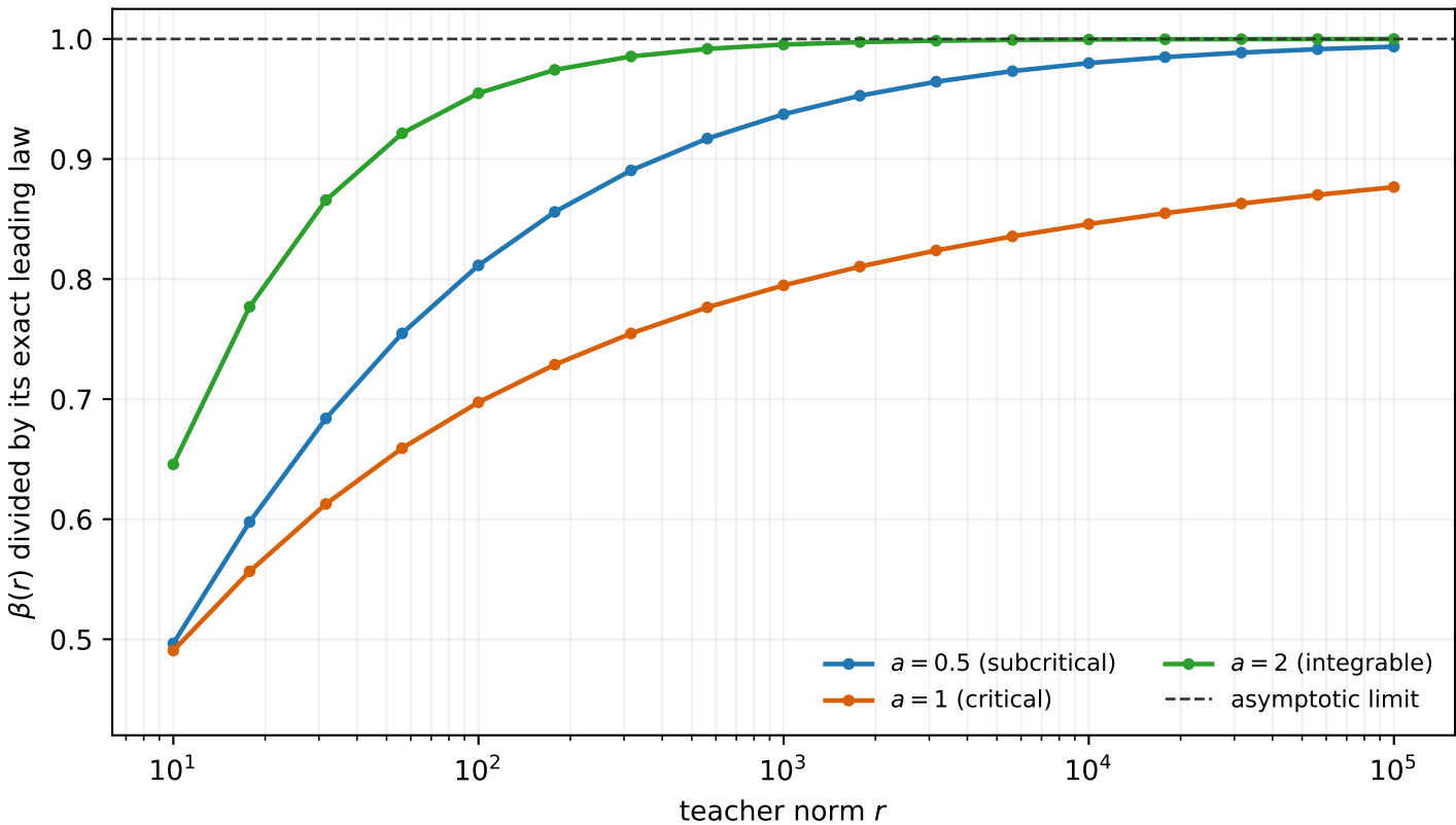
Three inverse-radius phases ( d = 3, h = \sigma' )
