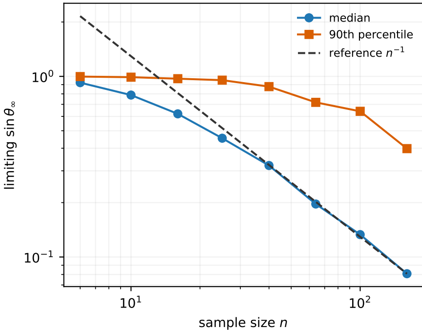
Order-statistic angle law ( d = 6 )
