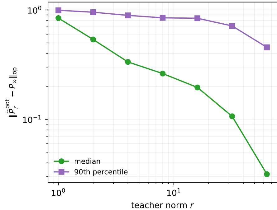
Spectral lexicography ( d = 5, n = 30 )
