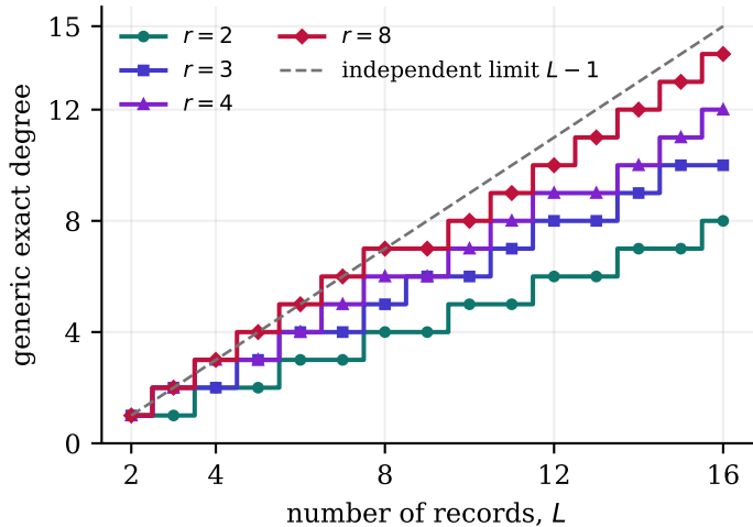
(b) Projective-span law
