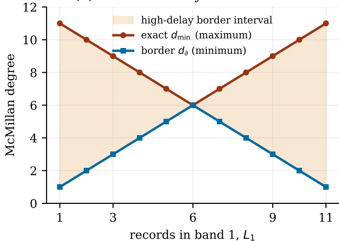
(a) Exact memory versus closure
