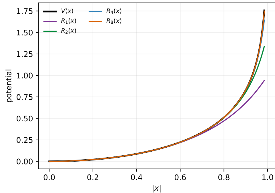
Nested Gauss--Stieltjes lower hierarchy
