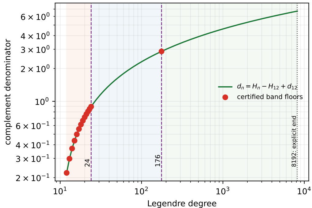
Mode-sensitive Schur denominators at a = 0.72
