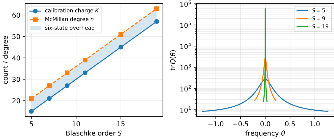
Figure 1: Left: the explicit irreducible six-port construction has calibration charge K_S = 3S and analytically derived McMillan degree n_S = 3S+6 , a constant six-state overhead above the universal lower bound. Right: the phase volume, fixed by the degree of each network and increasing from 21 to 63 across the shown family, becomes increasingly concentrated into a high Wigner–Smith peak as r_S approaches the unit circle. The frequency windows differ by S so the peak shapes remain visible.
