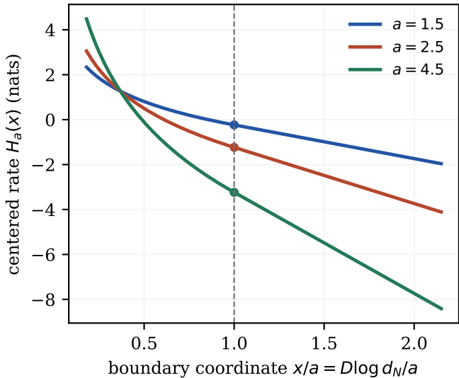
Universal matched boundary profiles
