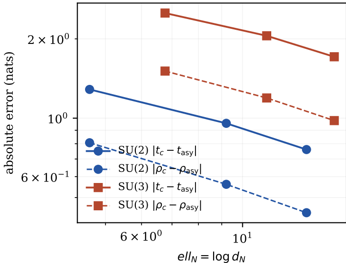
Exact Weyl-series contact diagnostics
