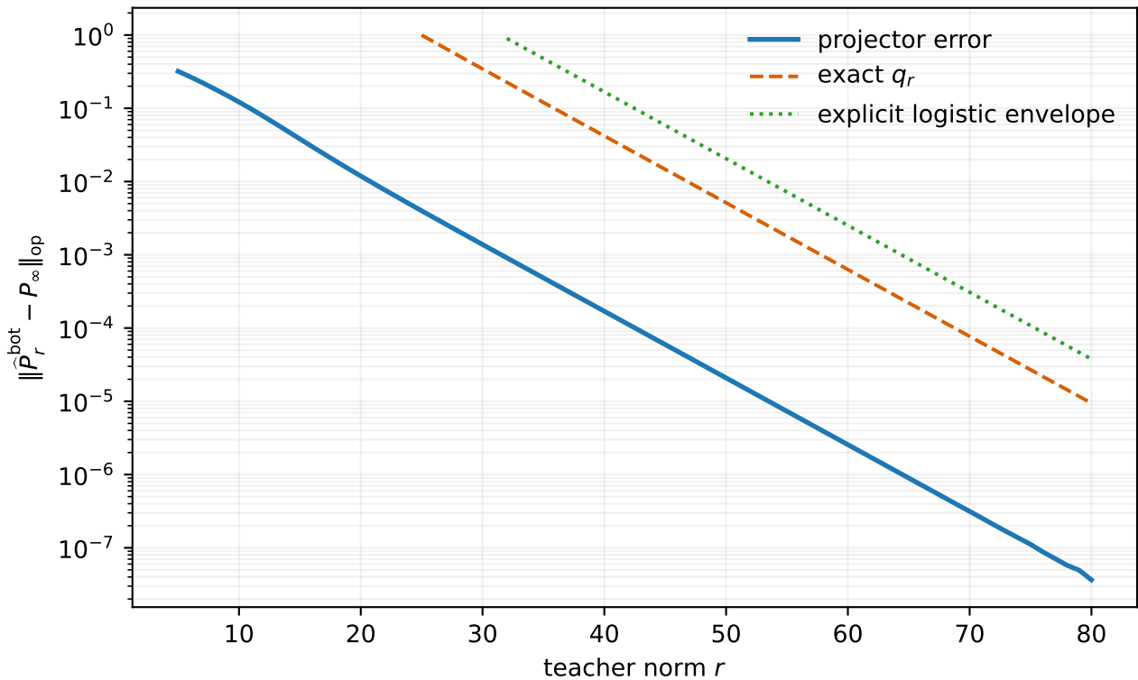
Finite-saturation certificate ( d = 5, n = 30 )
