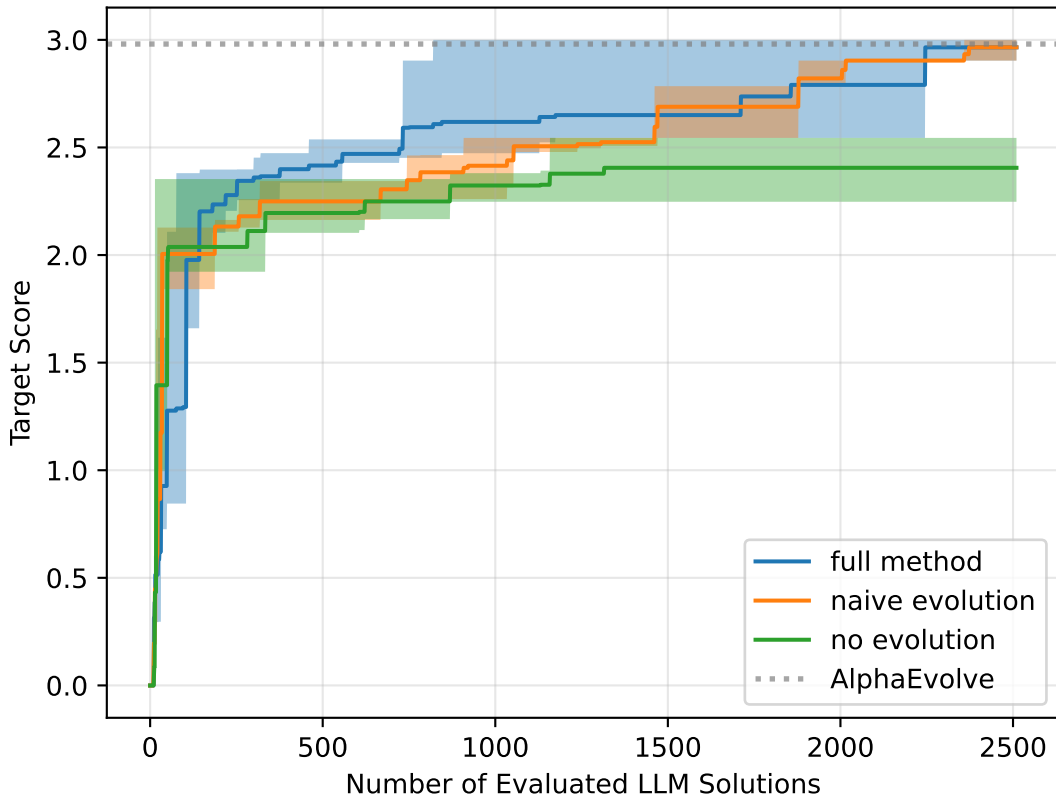
Component ablation for CirclePackingSquare( n=26 )
