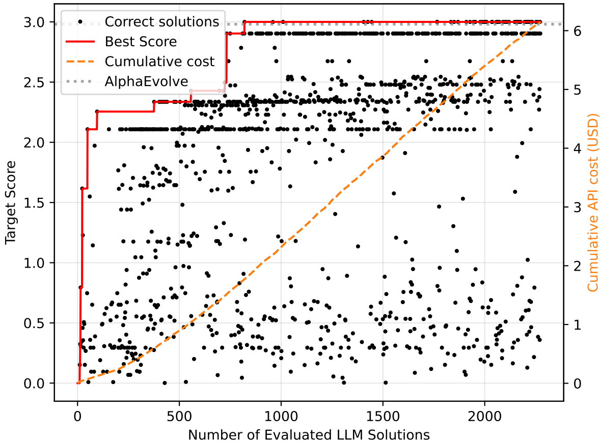
Solution history for CirclePackingSquare(n=26) with Qwen3-Coder-30B
