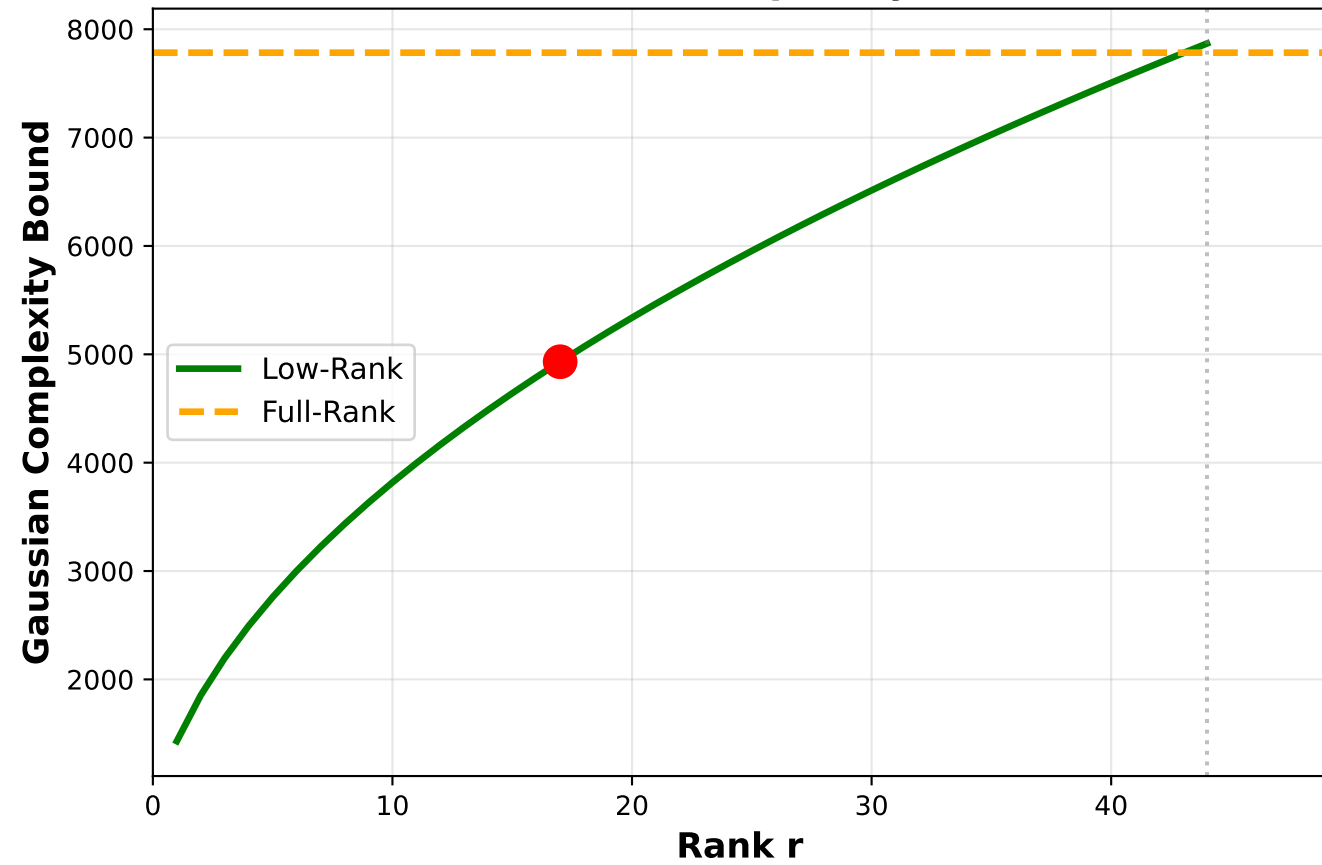
(B) Gaussian Complexity Bounds
