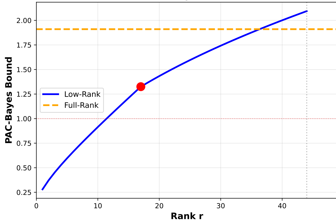
(A) PAC-Bayes Bounds
