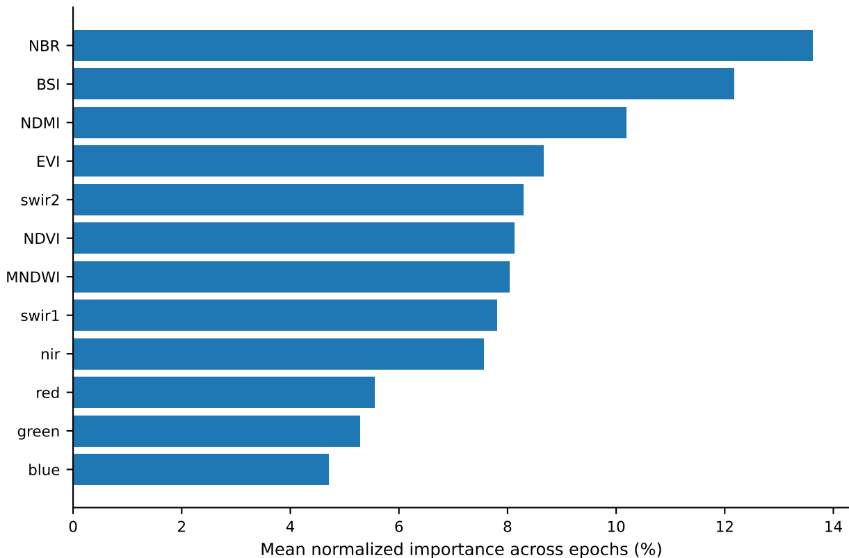
Random Forest predictor importance
