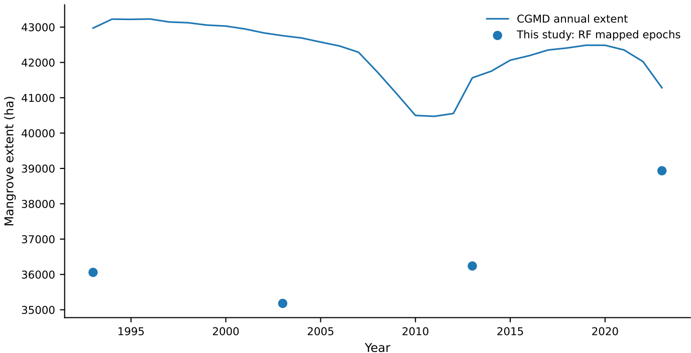
MMFR mangrove extent: study-specific RF snapshots and CGMD context
