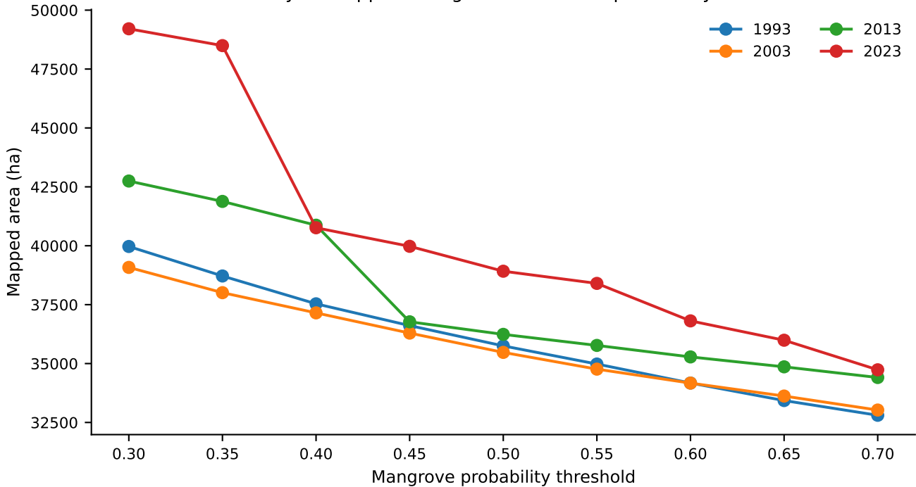
Sensitivity of mapped mangrove area to RF probability threshold
