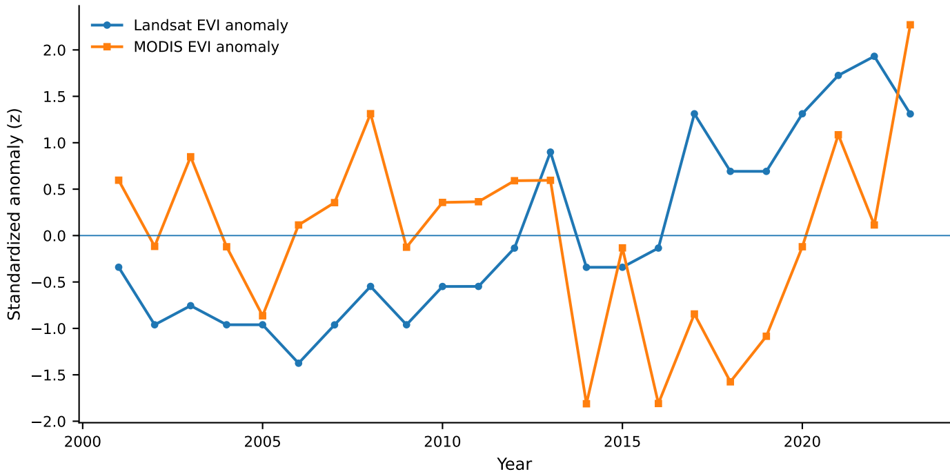
Cross-sensor EVI sensitivity, detrended \rho=0.34
