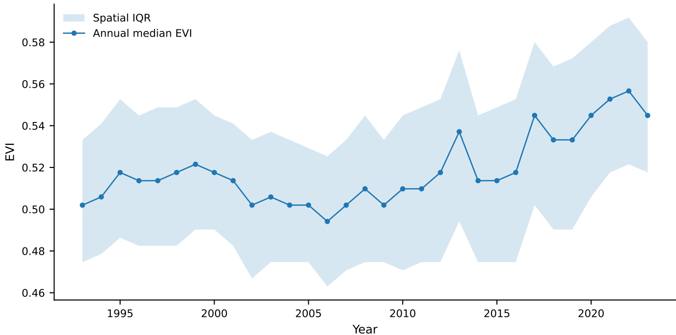
Annual mangrove greenness trajectory
