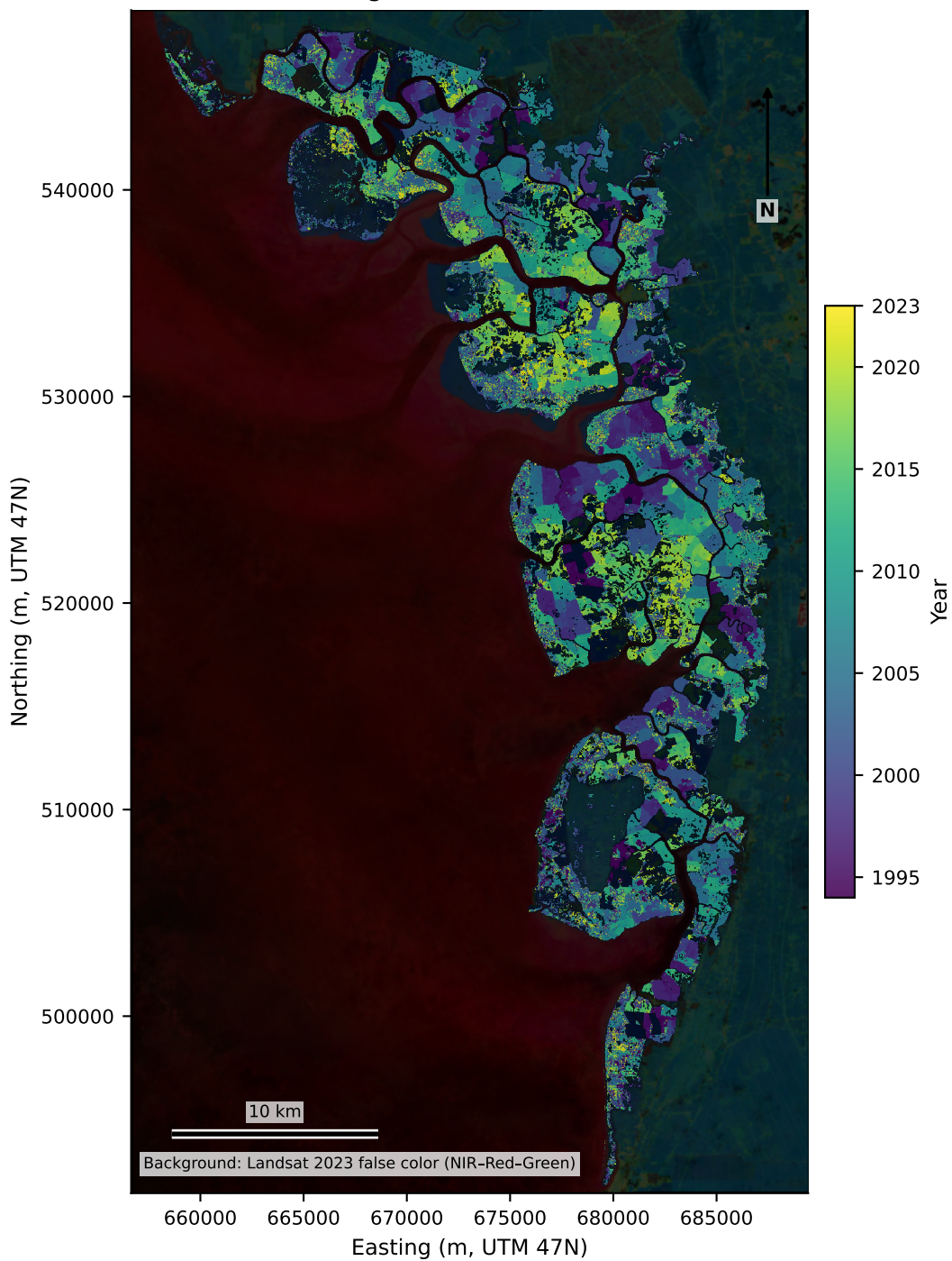
Year of largest annual NDMI decline
