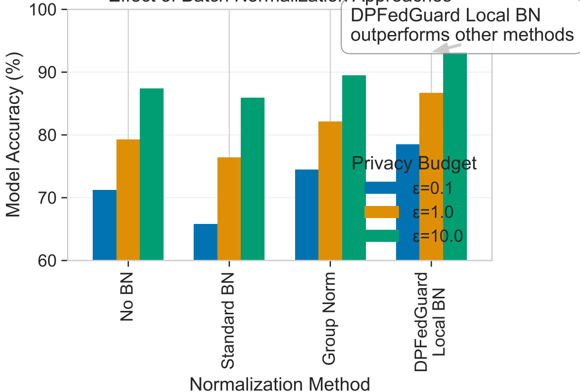
Effect of Batch Normalization Approaches
