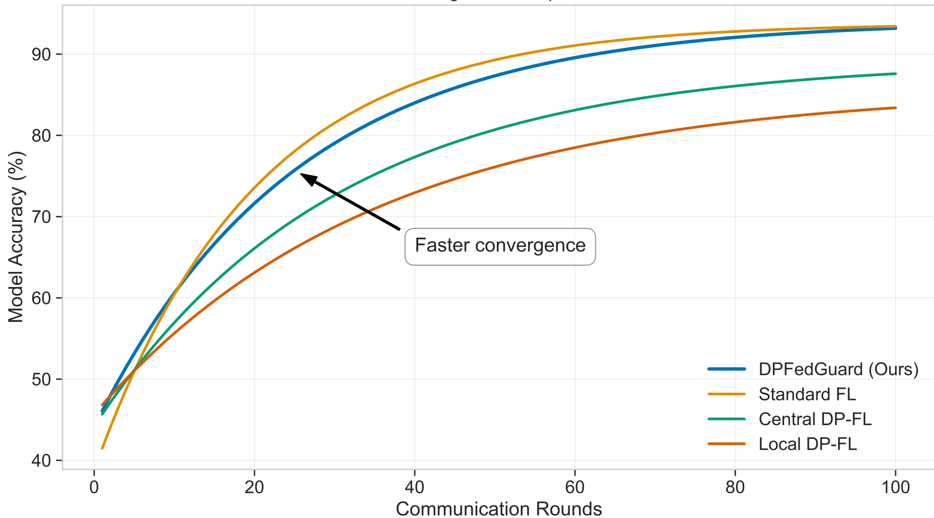
Convergence Comparison
