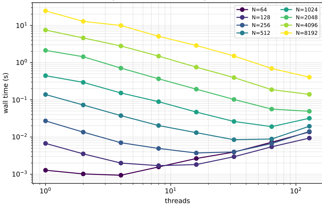
Paper I forward pass, Delta CPU (job 21181232) Optimal thread count depends on N
