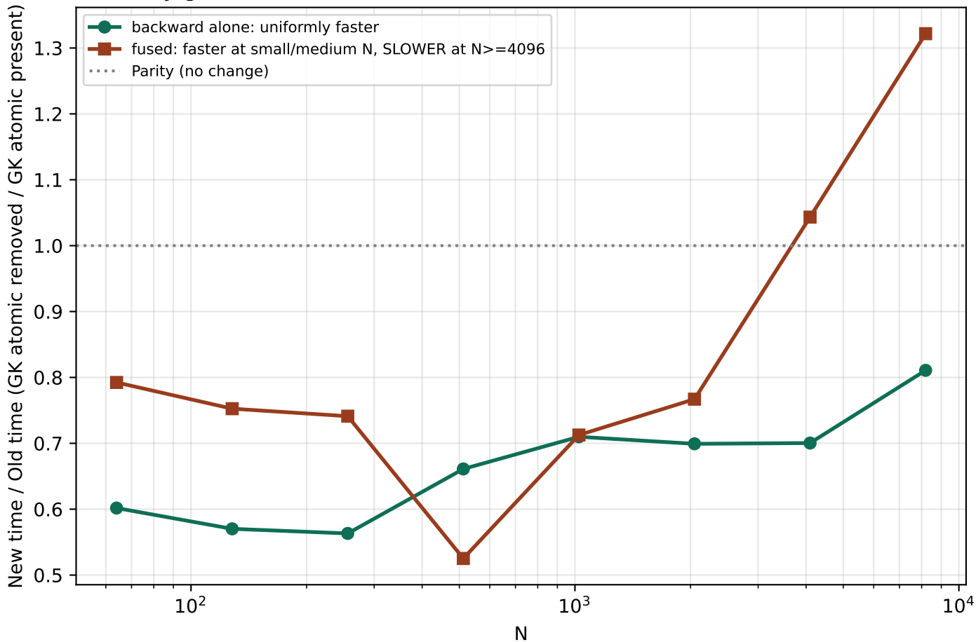
Removing GK's atomic too: real A100 results Uniformly good for backward alone; mixed for fused (net win still holds vs naive)
