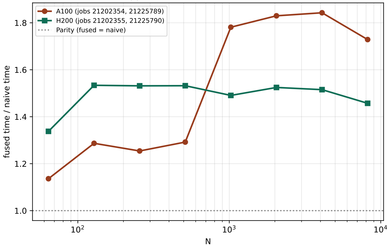
Paper II GPU: fused is SLOWER than naive at every size (opposite of the CPU N=4096 result)
