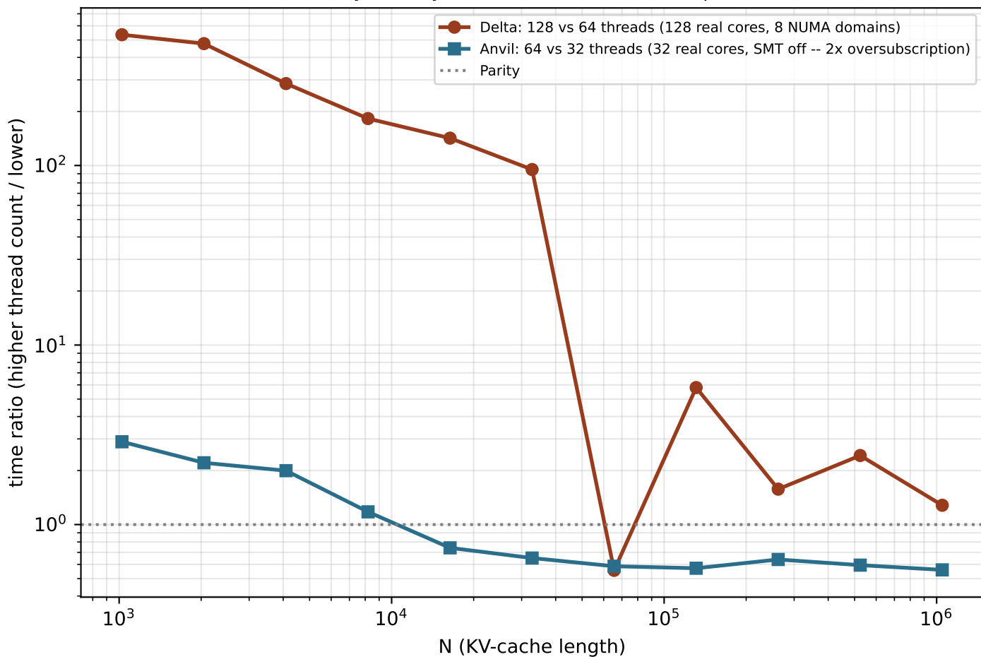
Paper III decode: two clusters, two different penalties Delta: NUMA memory-locality (535x). Anvil: oversubscription (<3x, reverses)
