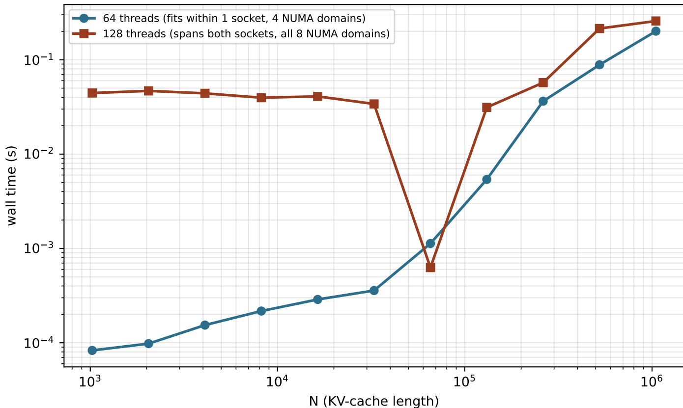
Paper III decode, Delta CPU (job 21249667): 128-thread NUMA penalty Up to 535x slower at small N -- resolves once N amortizes cross-NUMA cost
