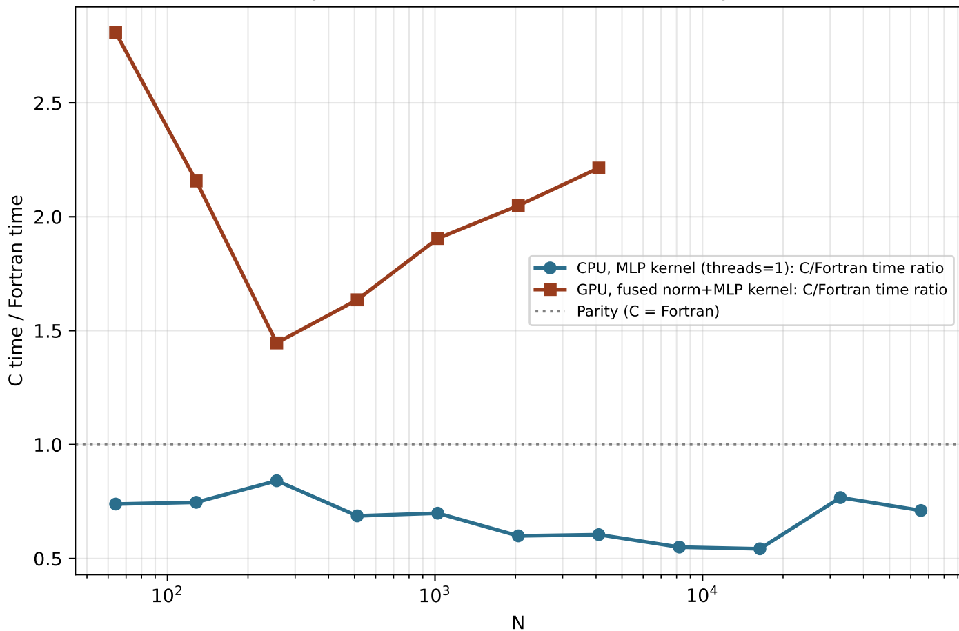
Paper IV: C vs Fortran runs in OPPOSITE directions on CPU vs GPU CPU: C consistently faster (ratio<1). GPU: C consistently slower (ratio>1).
