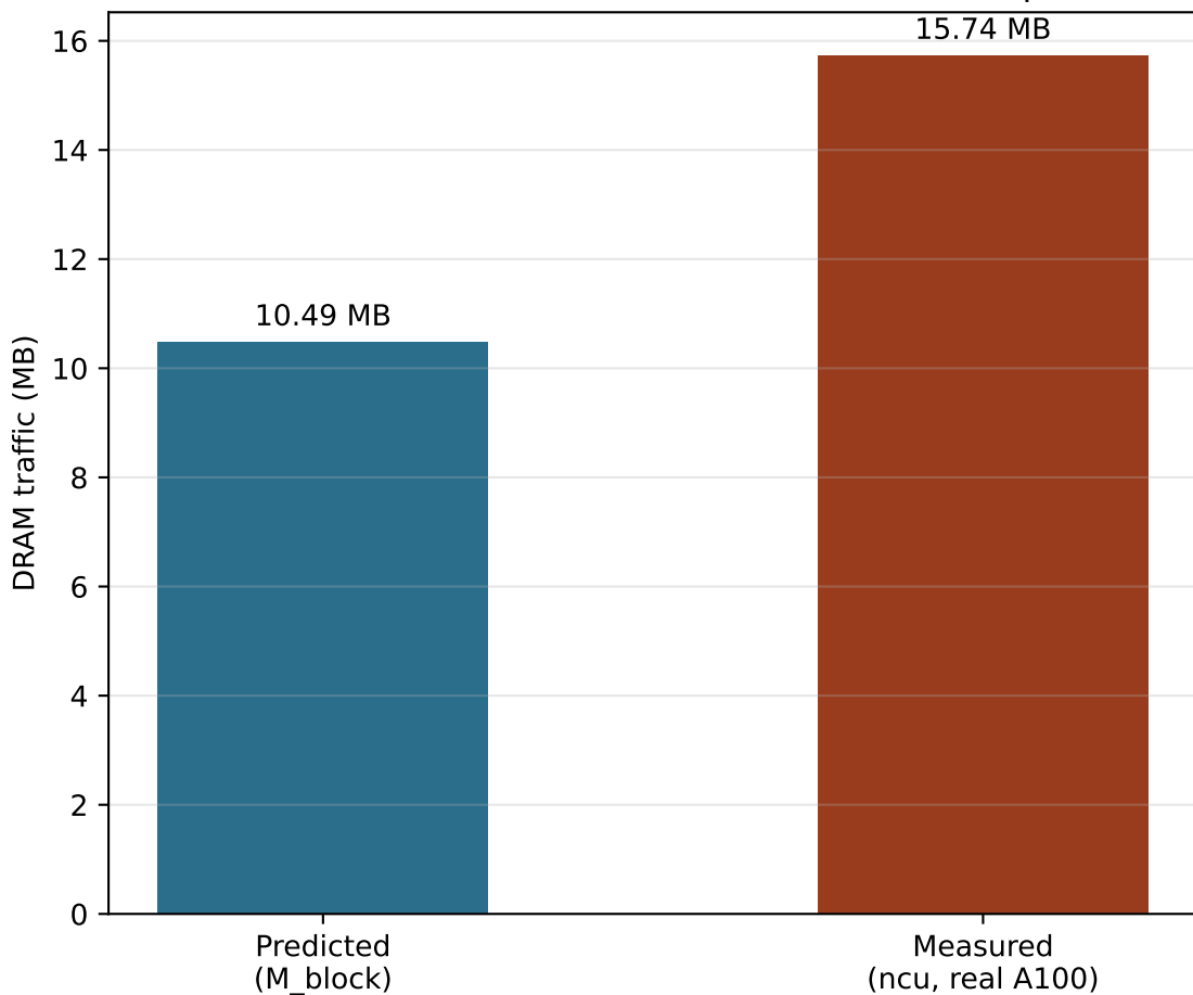
Paper IV: M_{block} real DRAM traffic validation B=2, N=256, D=64, DFF=256 -- measured is 1.50x predicted
