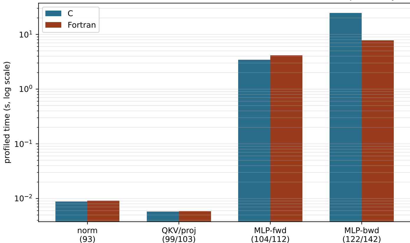
C vs Fortran, per-kernel profiled time at N=1024 (job 21299927) MLP-backward dominates both totals; C is 3.17x slower there specifically
